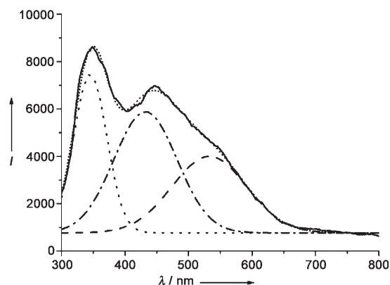
Figure 5. PL spectrum of the porous \text{Si}_3\text{N}_4 membrane obtained after nitridization for 4 h. —: experimental spectrum; ----, -.-, ···: component peaks; ·····: calculated combination of component peaks.
